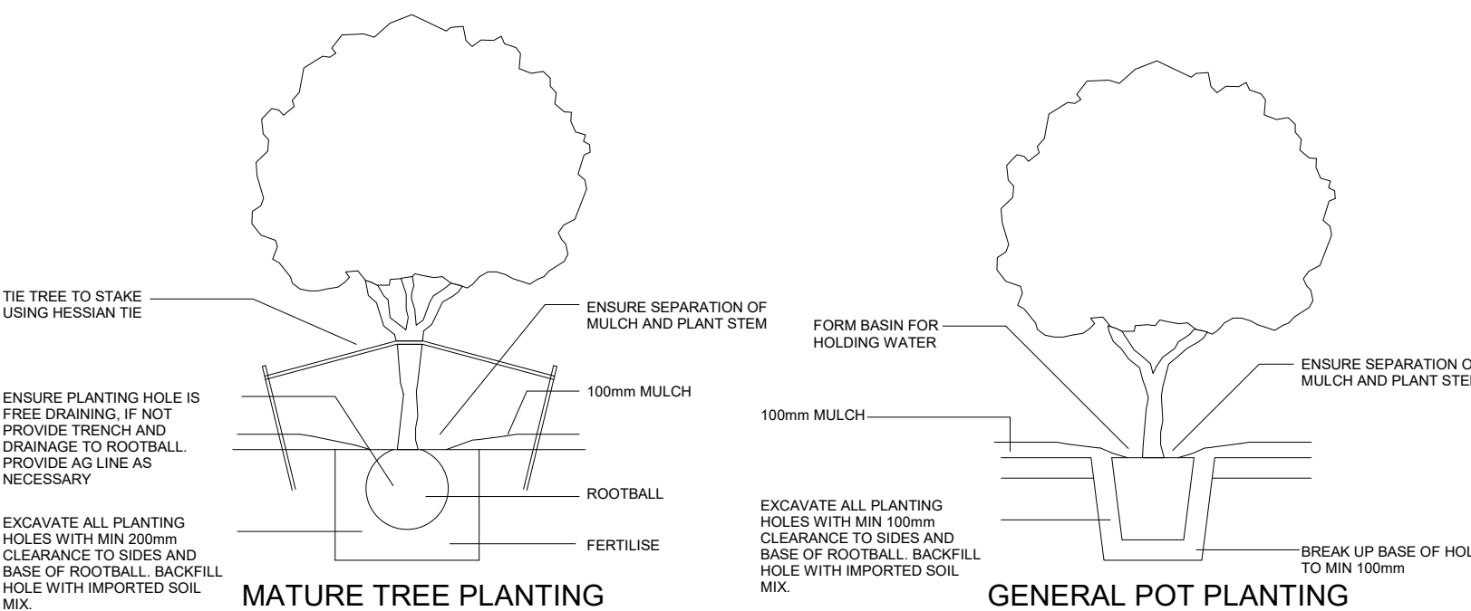
MATURE TREE PLANTING
