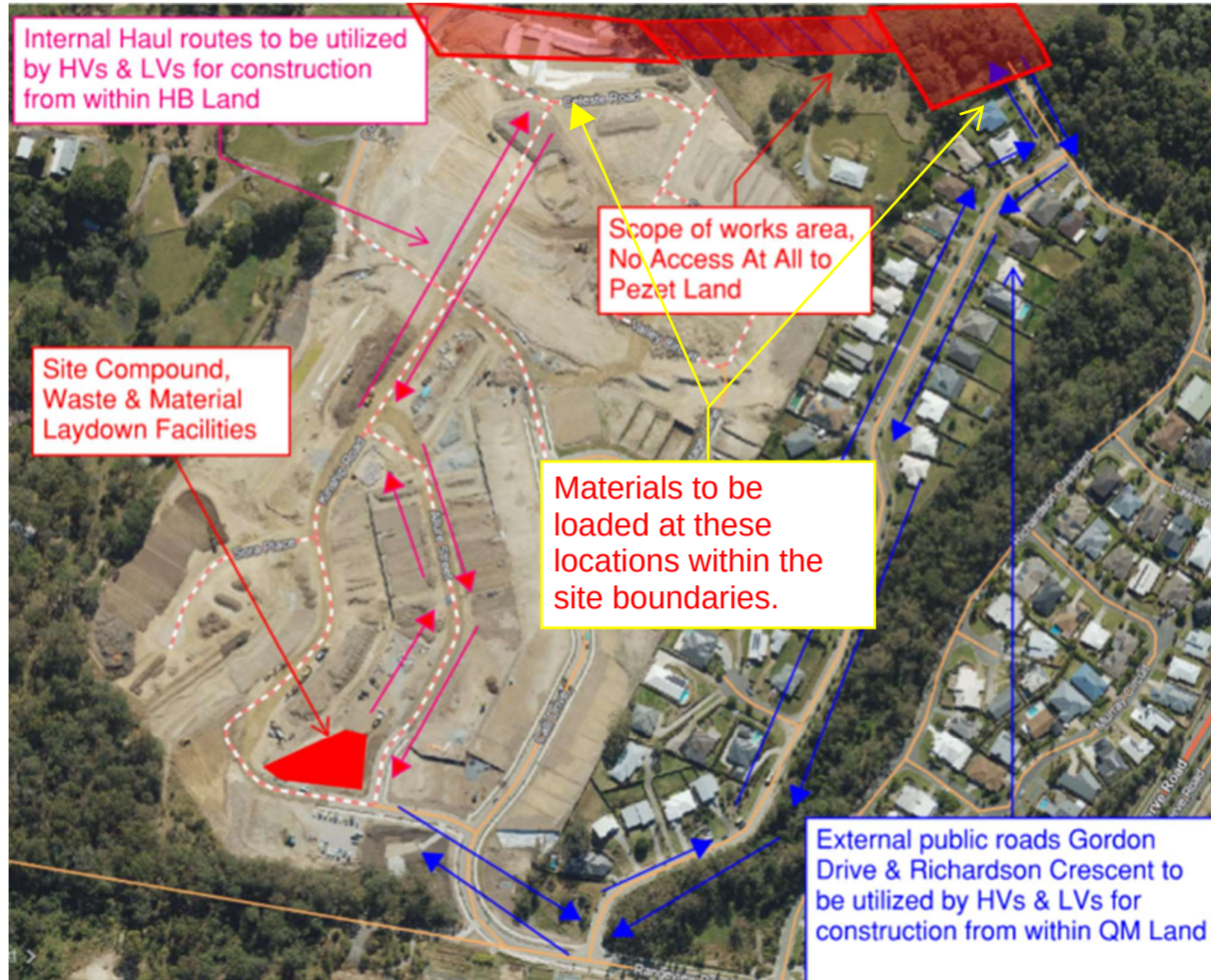
Site plan of proposed facilities & layout within the stage.
