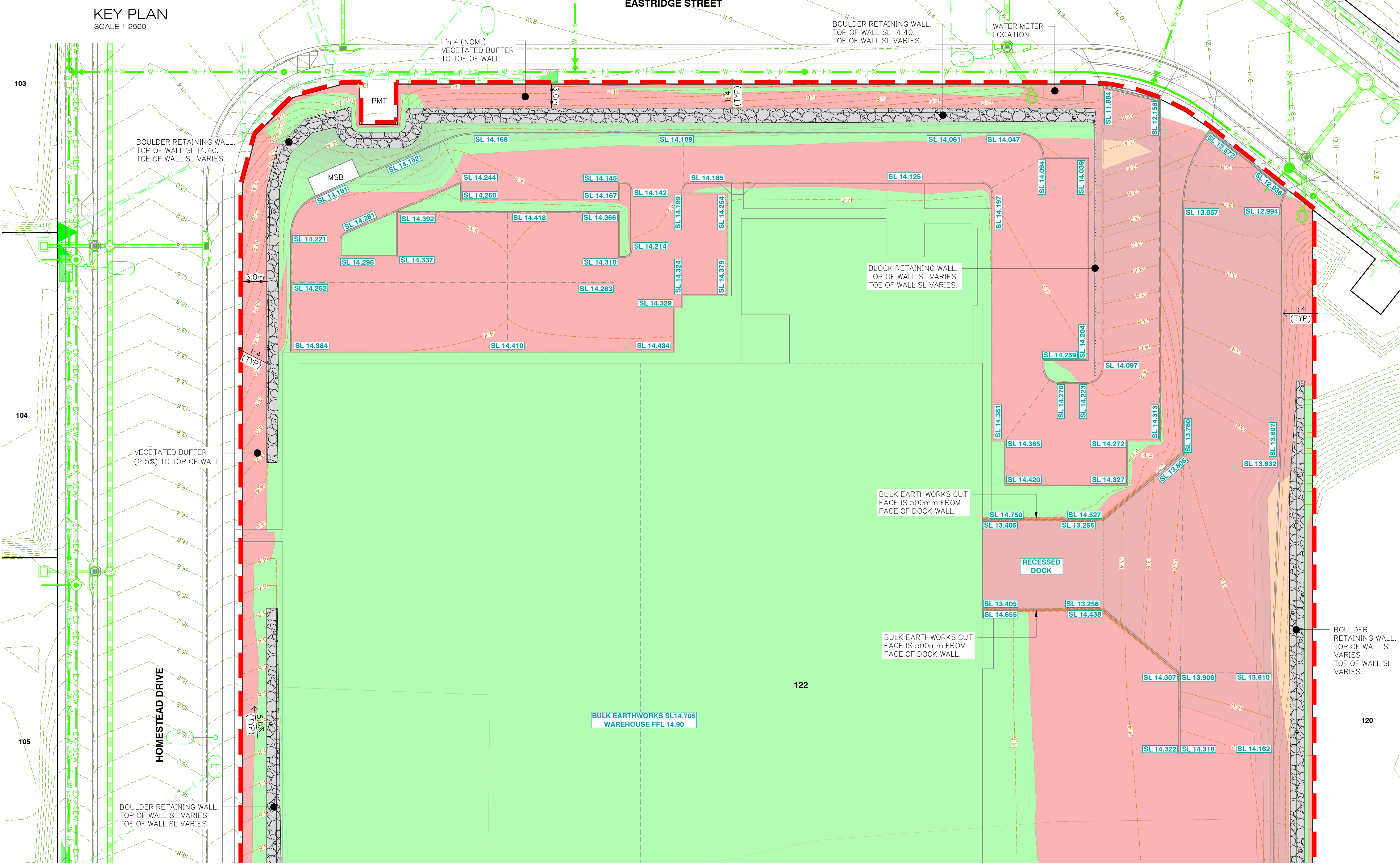
BULK EARTHWORKS CUT & FILL LAYOUT PLAN SHEET 1 OF 2
