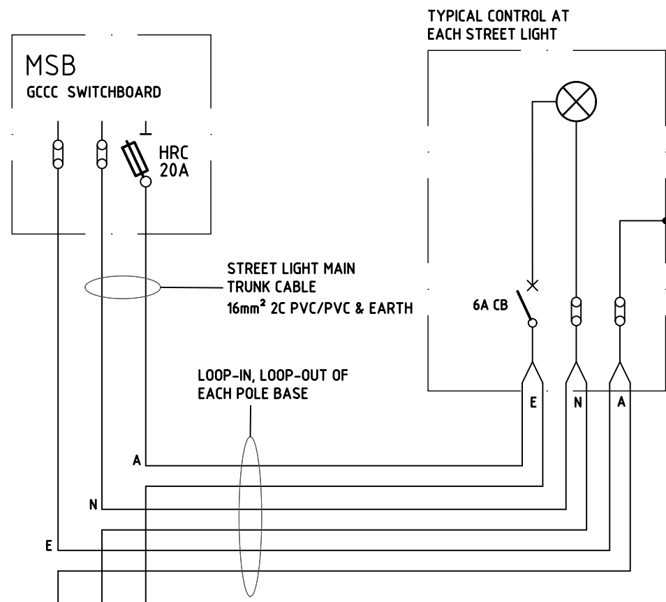
TYPICAL STREET LIGHT POLE INSTALLATION SCHEMATIC
