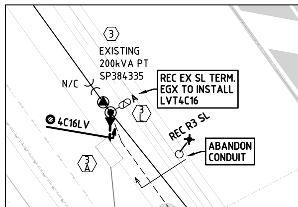
STN 3 - DETAIL 'B' SCALE 1:100 @ A1
