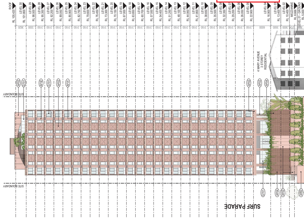
SOUTH ELEVATION
