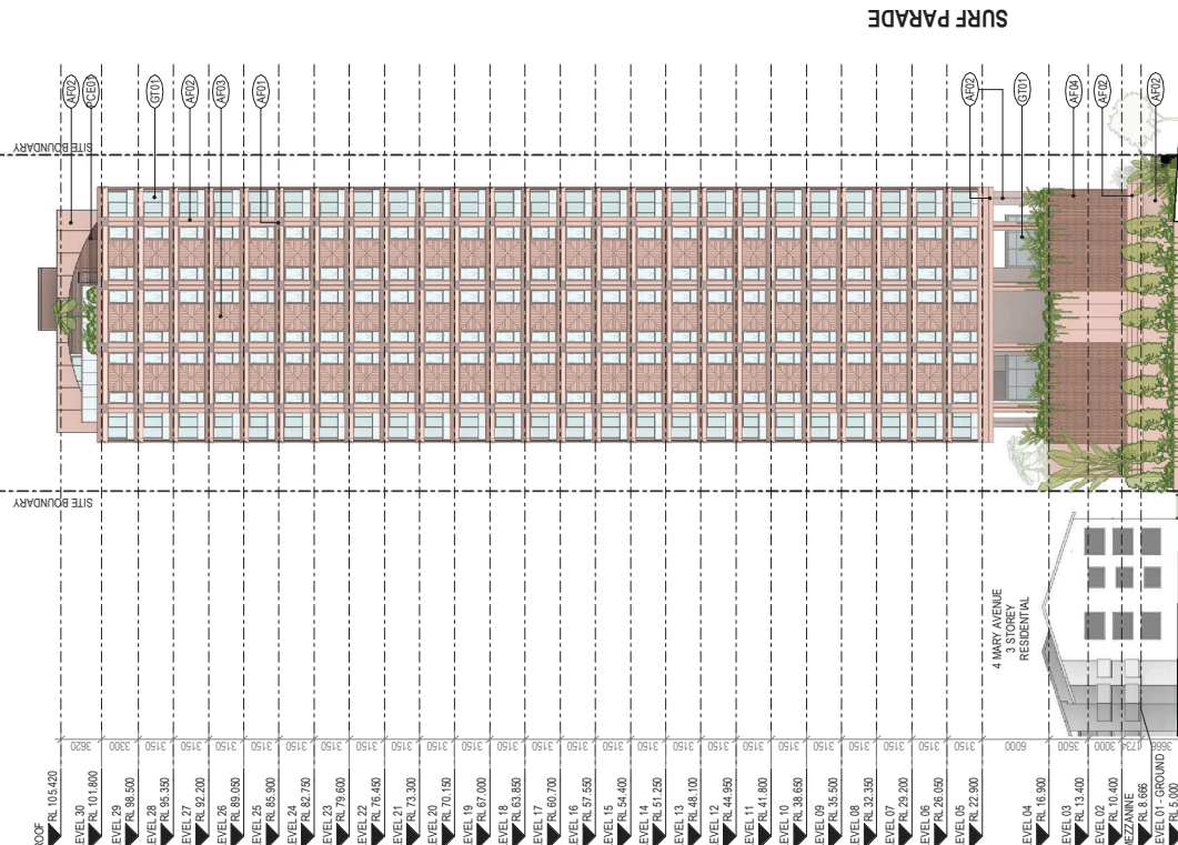
NORTH ELEVATION
