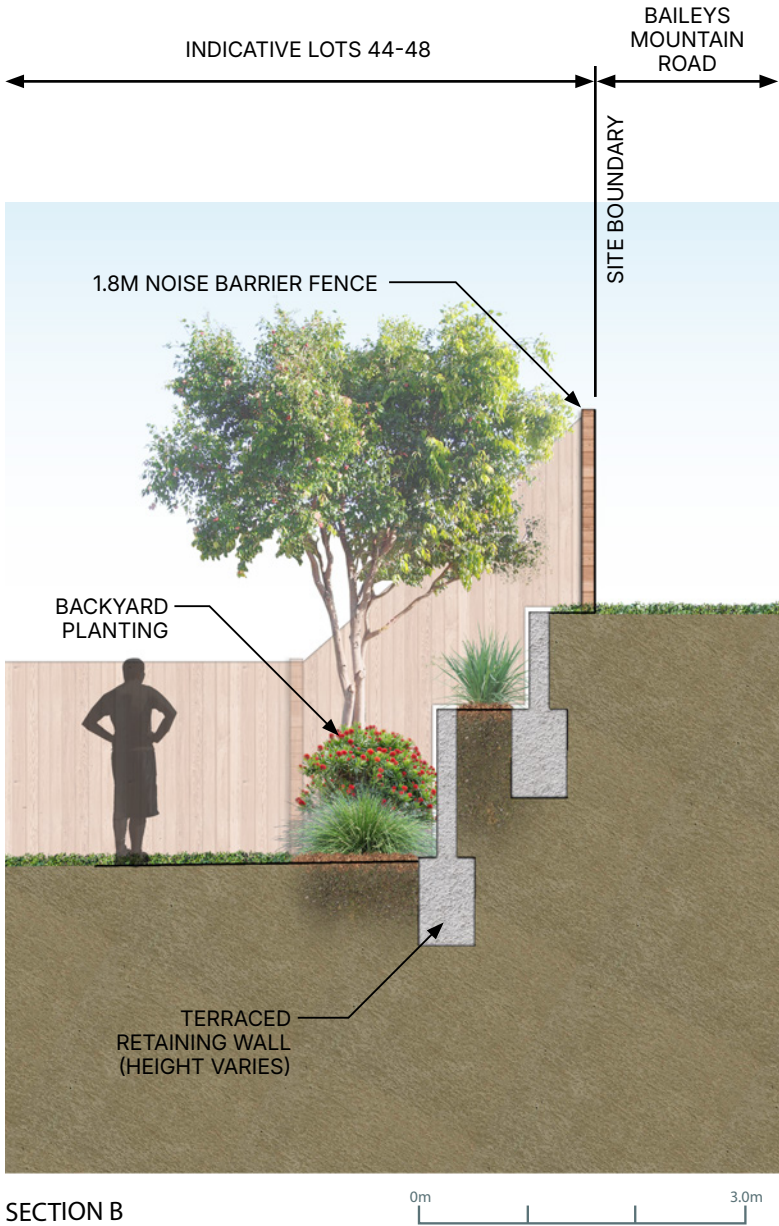
SECTION B
