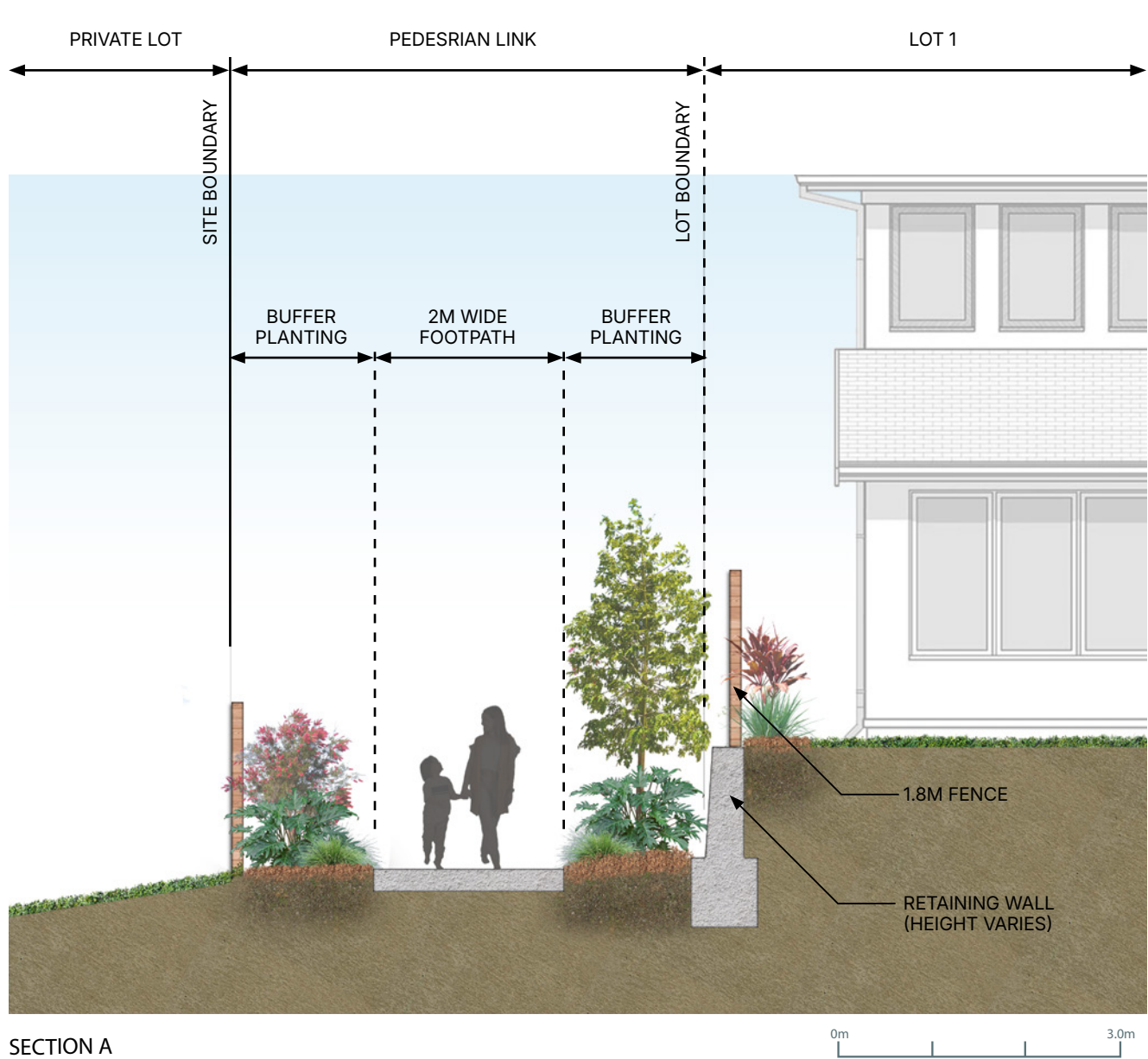
SECTION A
