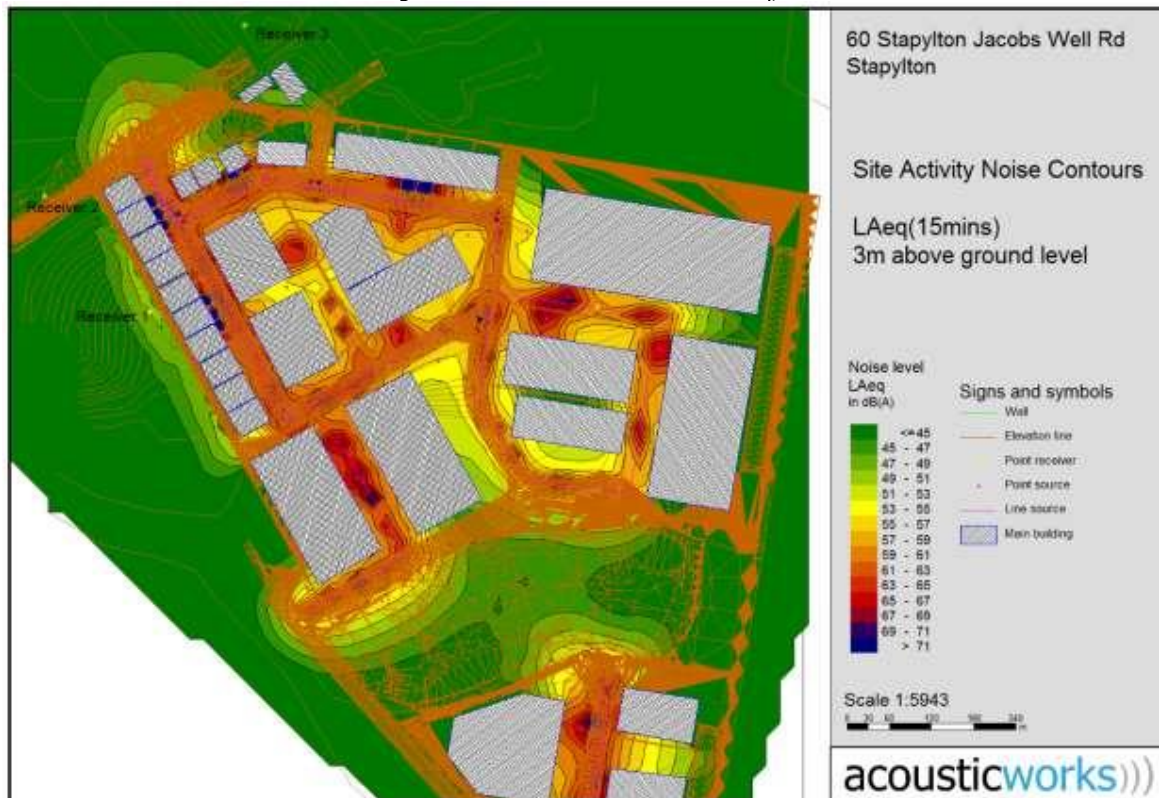
Figure 3: Predicted Noise Levels - LAeq, T
