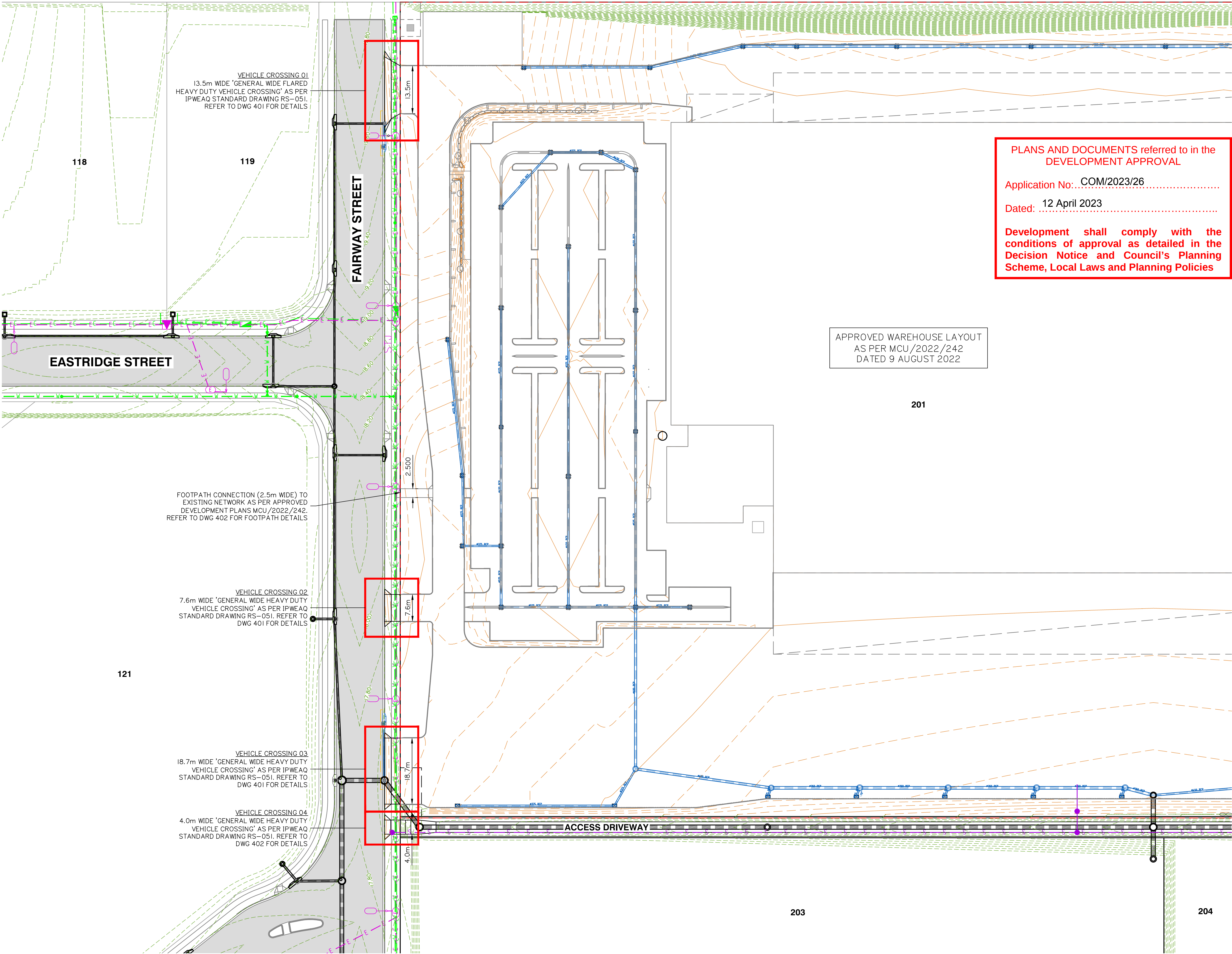
SITE LAYOUT PLAN
