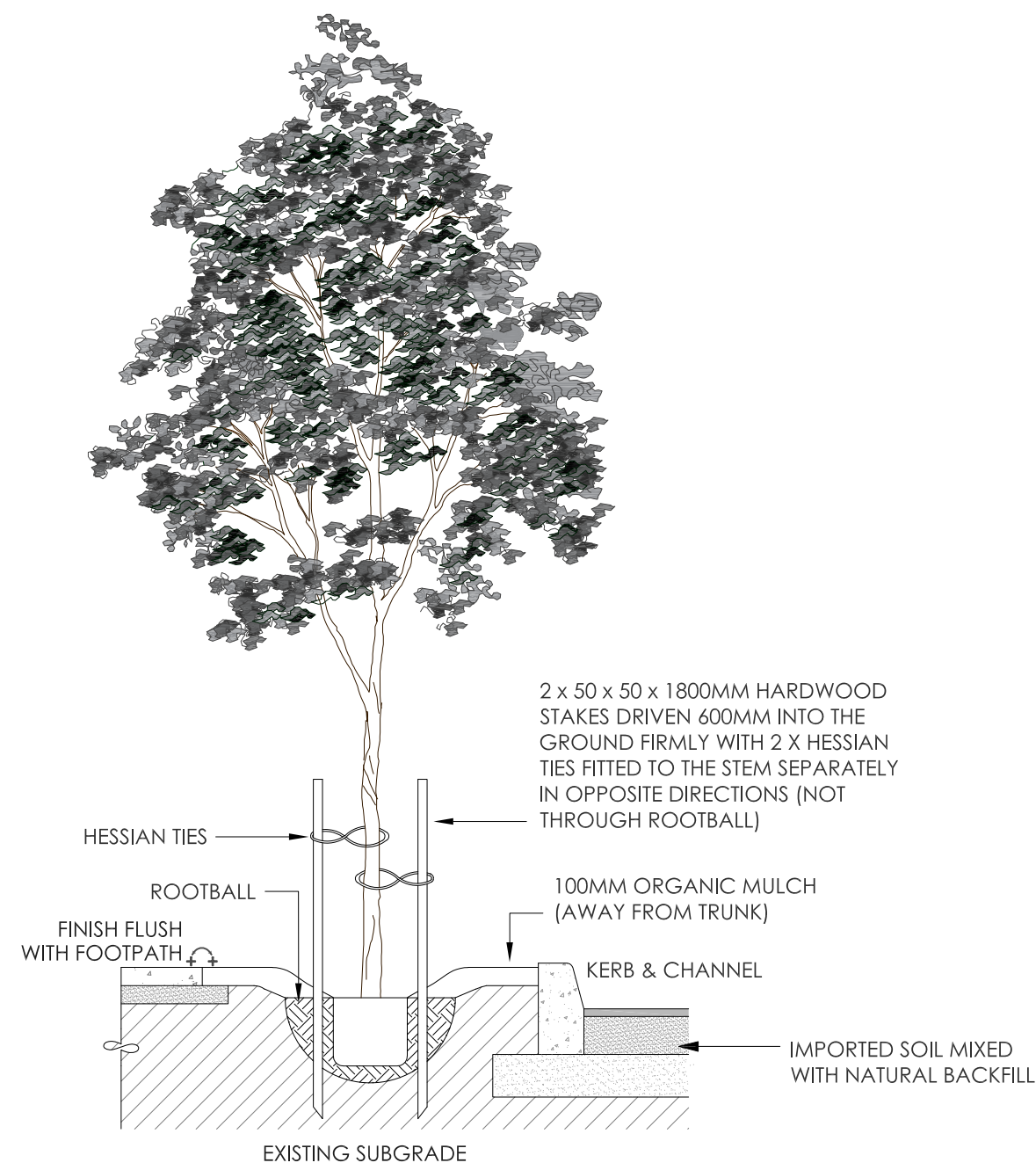
LD01 STREET TREE PLANTING DETAIL SCALE NTS (INDICATIVE)
