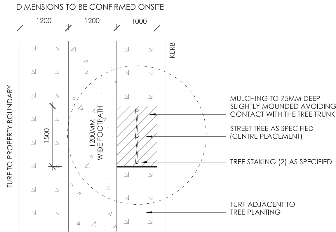
LD01 STREET TREE PLANTING DETAIL SCALE NTS (INDICATIVE)
