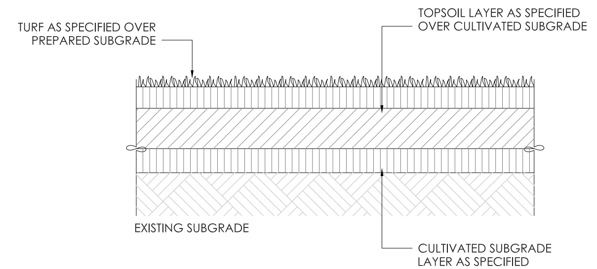
LD06 TURF DETAIL SCALE NTS
