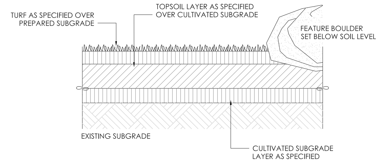
LD03 TURF + BOULDER DETAIL SCALE NTS
