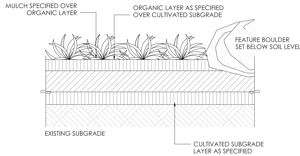
LD02 GARDEN + BOULDER DETAIL SCALE NTS (INDICATIVE)
